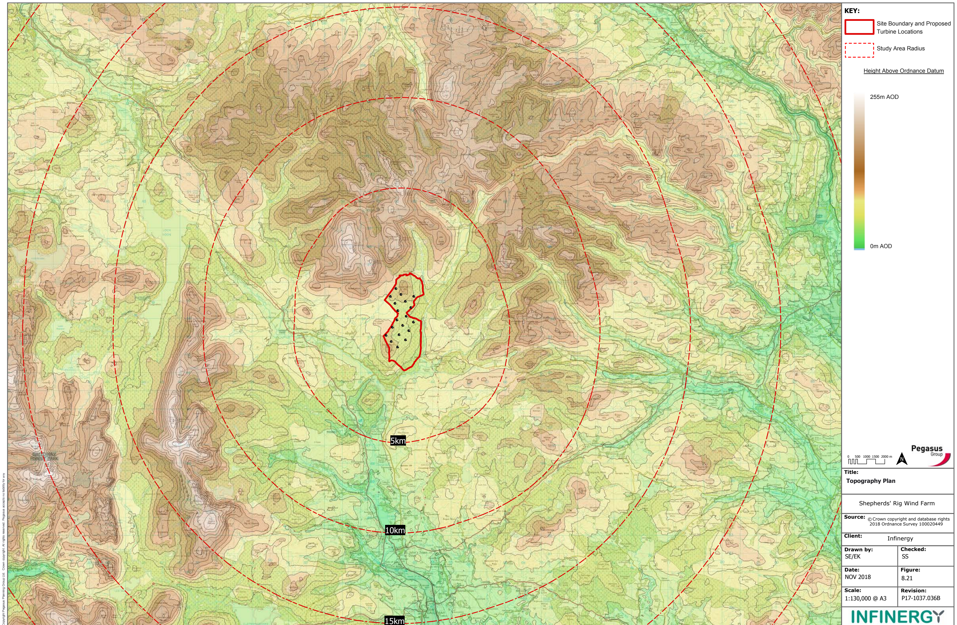
Figure 8.21: Topography Plan
